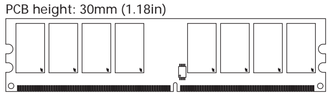
Figure 1: 240-Pin UDIMM (MO-237 R/Cs B and E)
